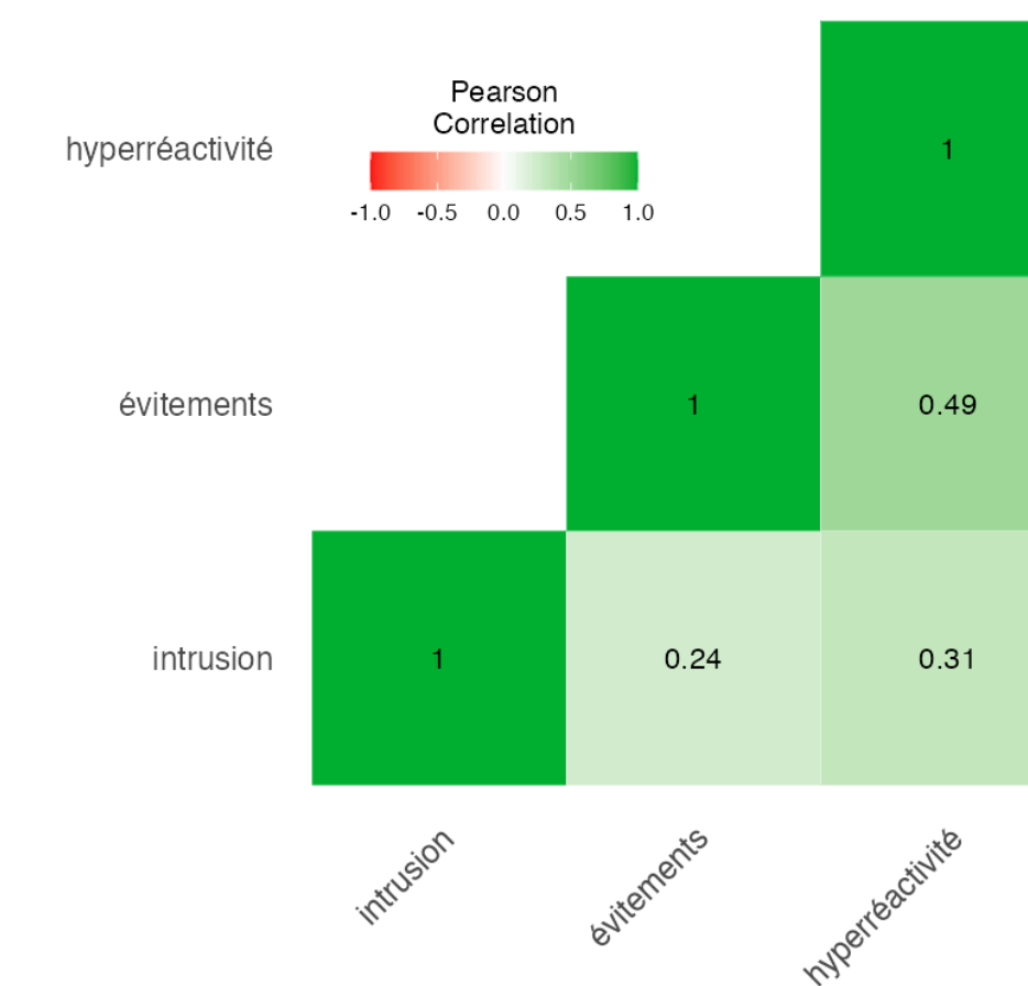
Correlation Heatmap
